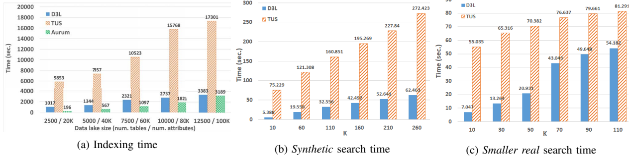
Fig. 6: Indexing and searching performance
