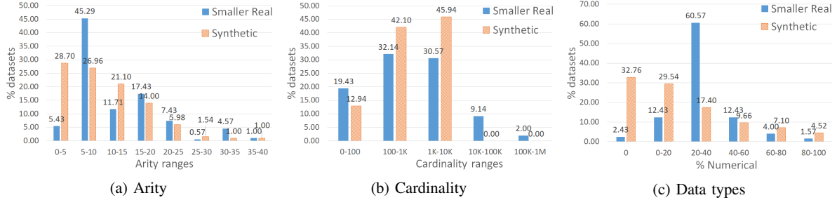
Fig. 2: Synthetic and Smaller Real statistics
